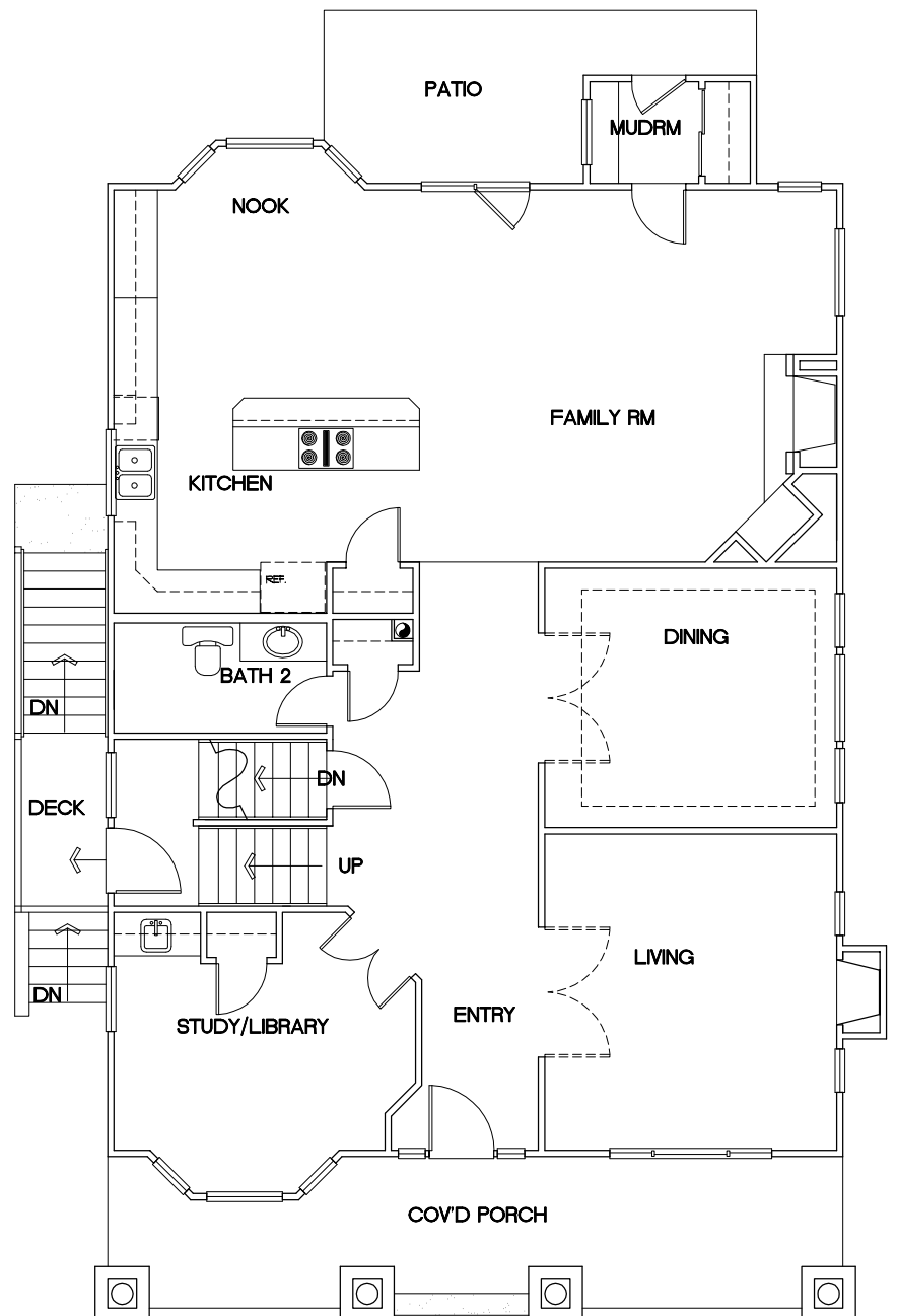
MAIN FLOOR PLAN 1618 S.F.
