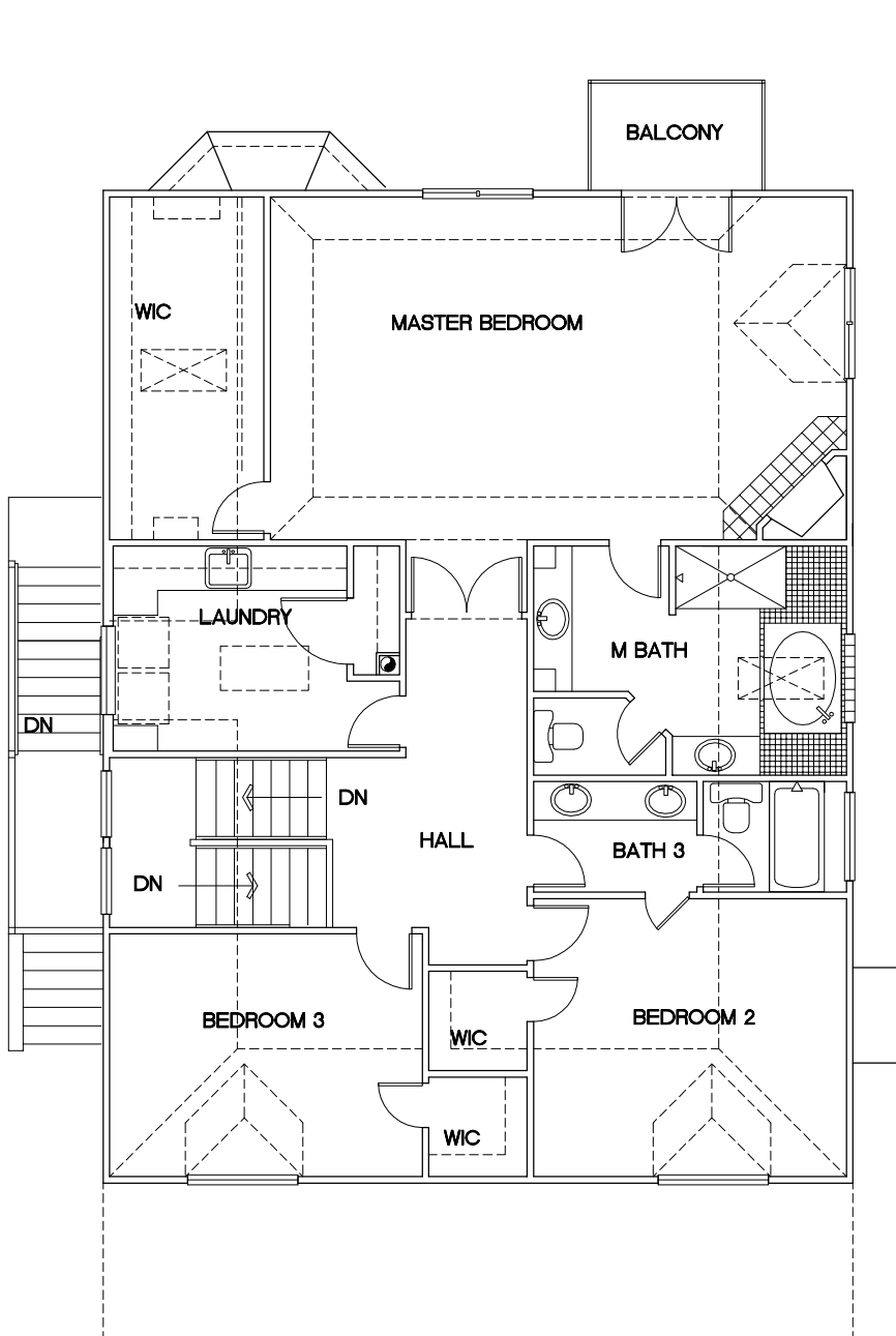
SECOND FLOOR PLAN 1452 S.F.
