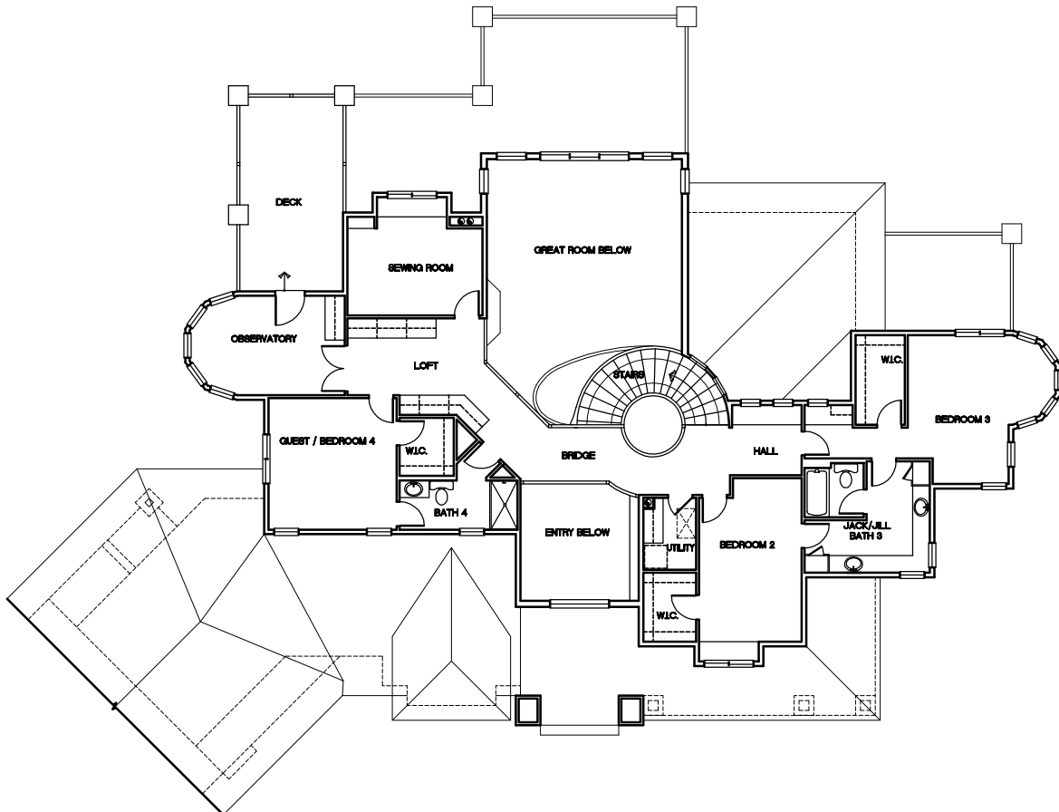
UPPER FLOOR PLAN 1,770 S.F.
