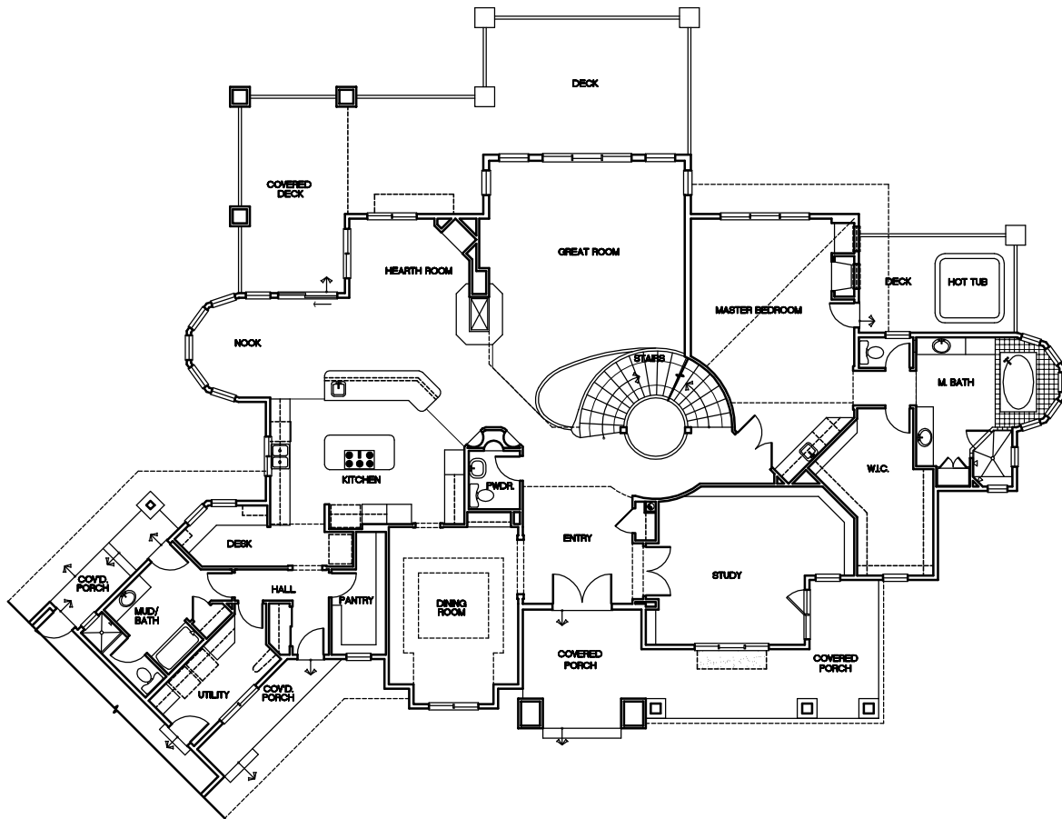
MAIN FLOOR PLAN 3,443 S.F.
