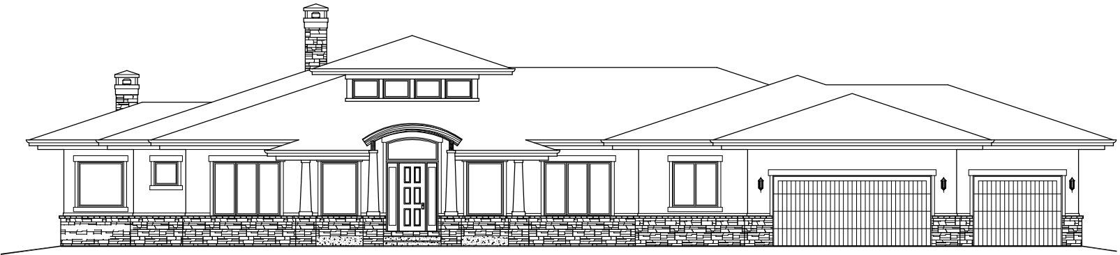
FRONT ELEVATION
